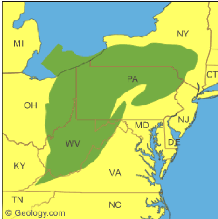
Map I. Map of Marcellus Shale
